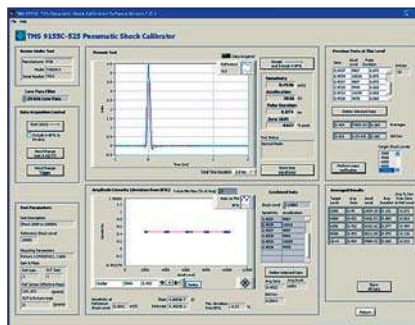
Figure 5. Calibration output results for a shock sensor tested from 2,000-10,000 g acceleration levels.
