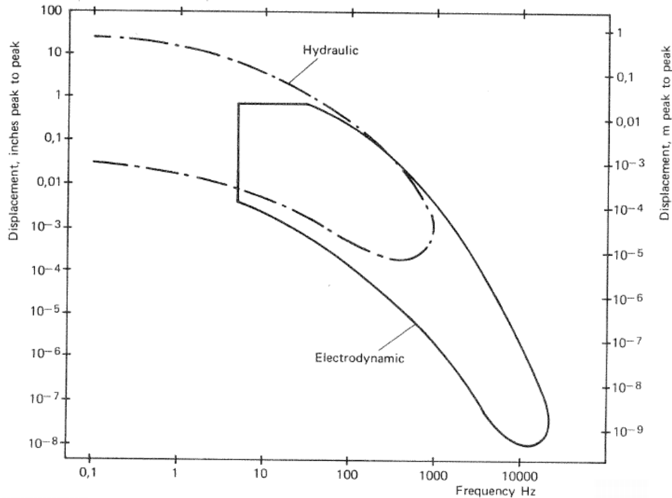
Useful operating regions of modern hydraulic and electro-dynamic vibration machines (after G.B. Booth)
